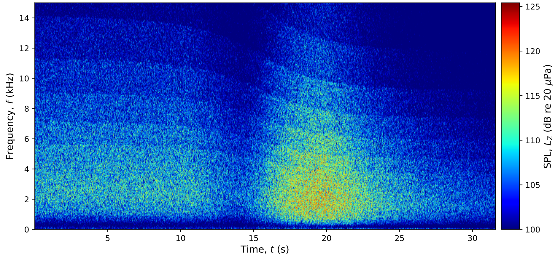
OUTPUT - Spectrogram of auralized BBN - emission - engine
