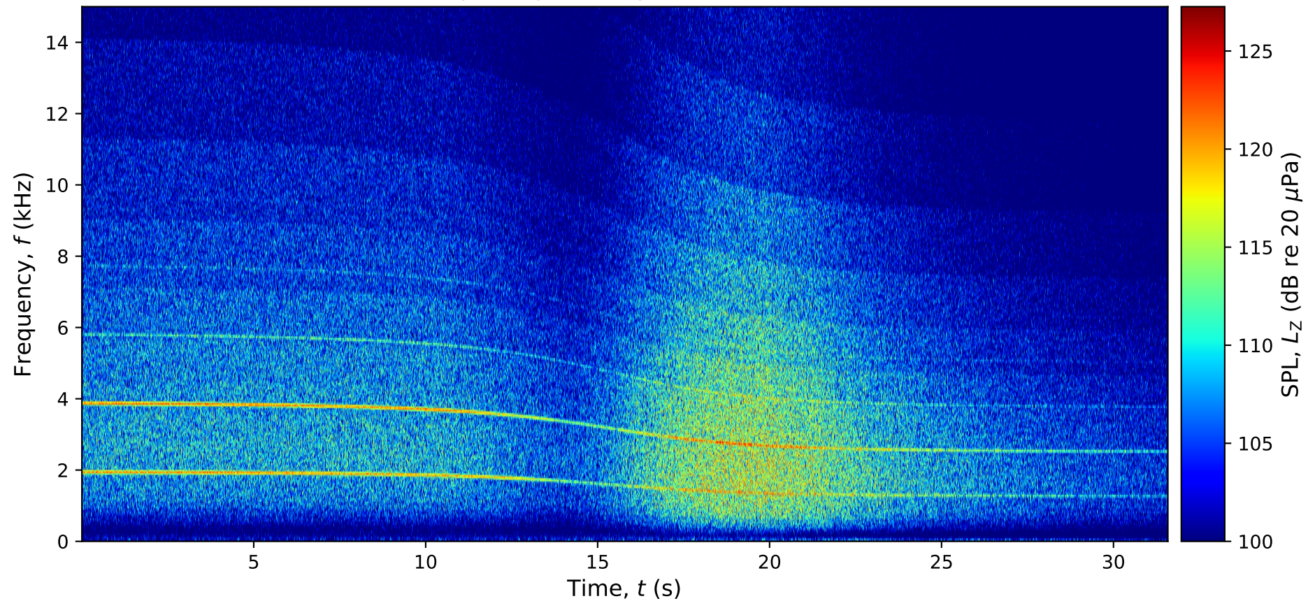
Spectrogram: Engine - emission
