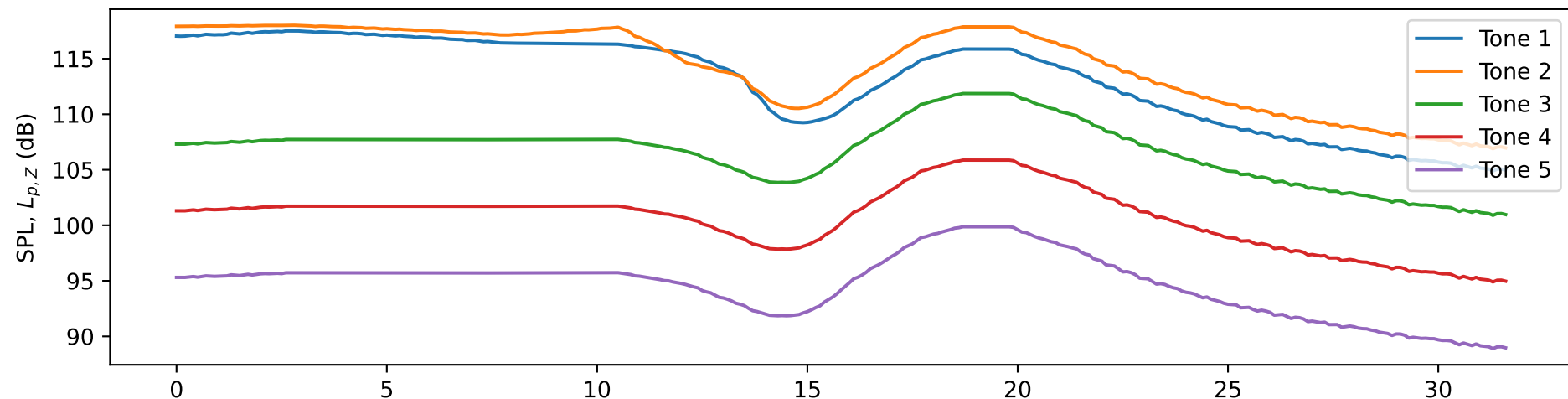
INPUT - Tonal content from PANAM - emission - fan_harmonics
