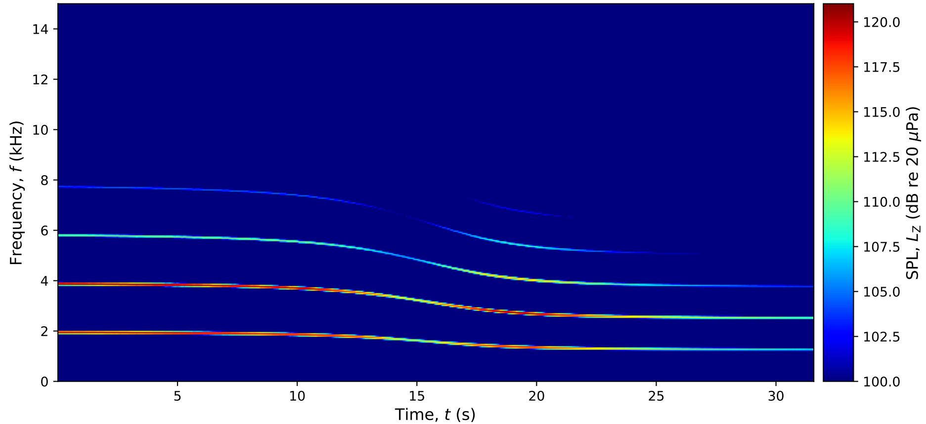
OUTPUT - Spectrogram of auralized tonal noise - emission - fan_harmonics
