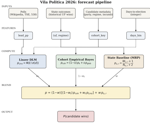
Figure 1: Forecast pipeline. Four data inputs (top row) each map to a primary engineered feature; features fan via right-angle bus into three estimators: Linzer dynamic linear ( p_{\text{Linz}} = \Phi(l / \sigma(d)) ), cohort empirical Bayes with global-prior shrinkage ( p_{\text{coh}} = (1-s)p_k + s p_{\text{glob}} ), and the MRP-style state baseline ( p_{u,r} = \frac{W_{u,r} + 1}{N_{u,r} + 2} ). The dashed connection denotes the secondary \sigma(d) pathway from days-to-election into the Linzer drift. The ensemble blend (yellow box) combines the three components with selected weights w_{\text{linz}} and w to produce the final candidate-level probability.
