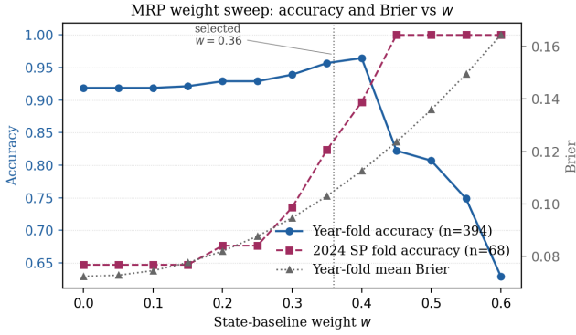
Figure 6: State-baseline weight sweep on the 394-event BR core. Year-fold accuracy (blue, left axis) is flat at the cohort+Linzer baseline of 91.88% for w \in [0.00, 0.15] , climbs through w = 0.36 to a maximum of 96.45% at w = 0.40 , then collapses sharply as the prior overrides the lead signal. The 2024 SP fold accuracy (purple, left axis) climbs monotonically from 64.71% at w = 0 to 100% at w \geq 0.45 . Year-fold mean Brier (grey, right axis) increases monotonically with w , reflecting the deliberate shift of probability mass away from extreme polls toward the state anchor; selective accuracy at w = 0.40 (Geifman and El-Yaniv 2017) absorbs this calibration cost.
