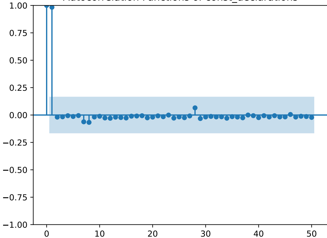
Autocorrelation Functions of const_declarations
