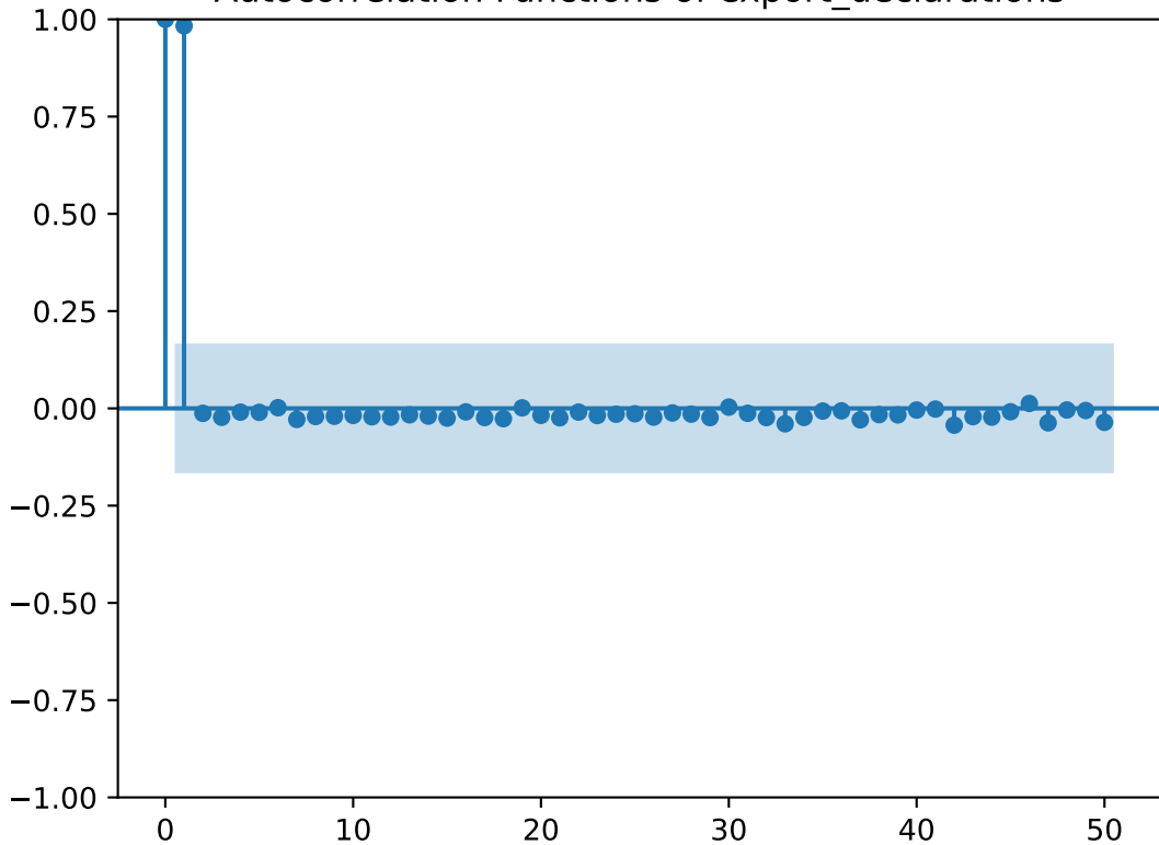
Autocorrelation Functions of export_declarations
