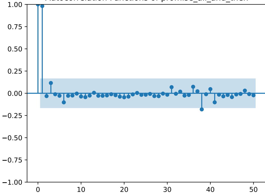
Autocorrelation Functions of promise_all_and_then
