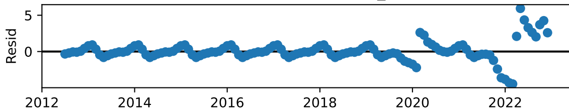
Decomposition of big_int
