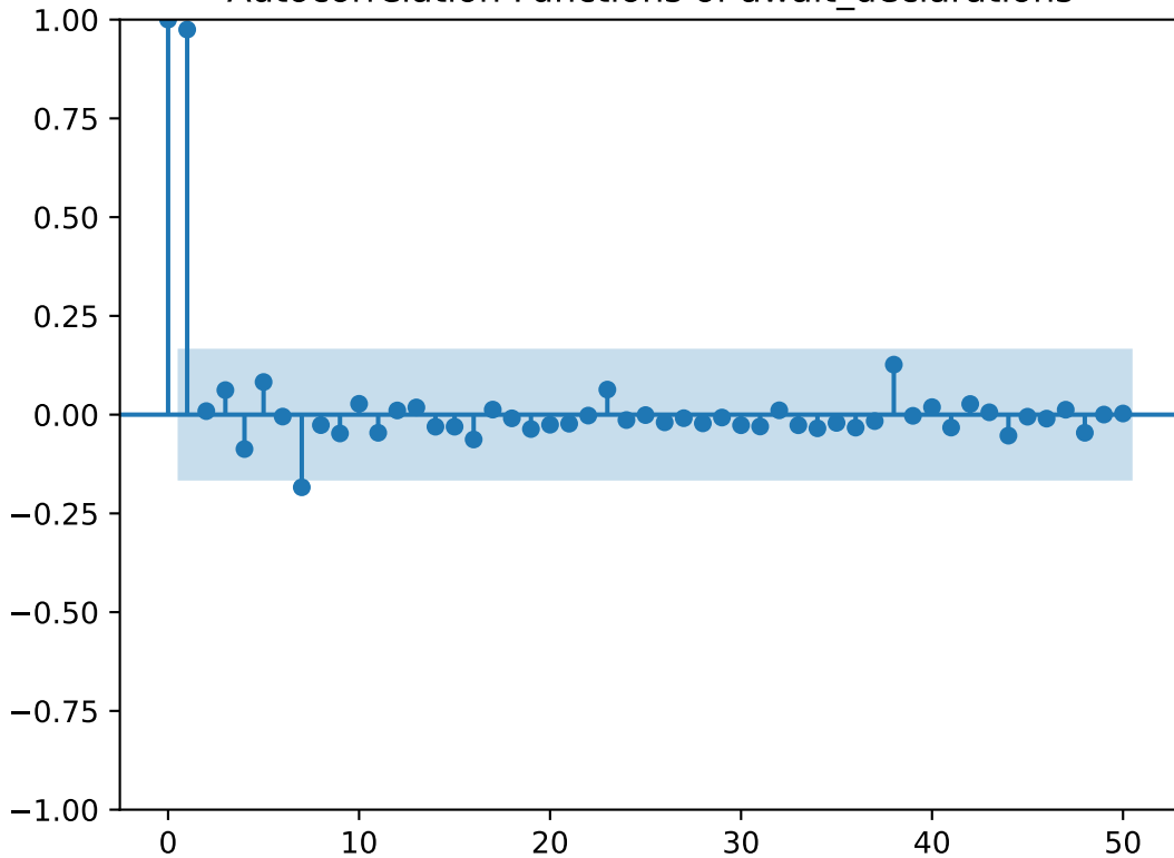
Autocorrelation Functions of await_declarations
