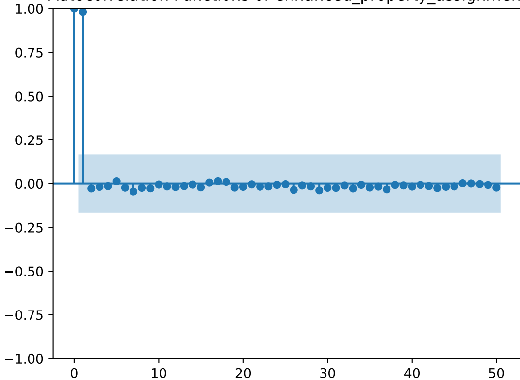
Autocorrelation Functions of enhanced_property_assignment
