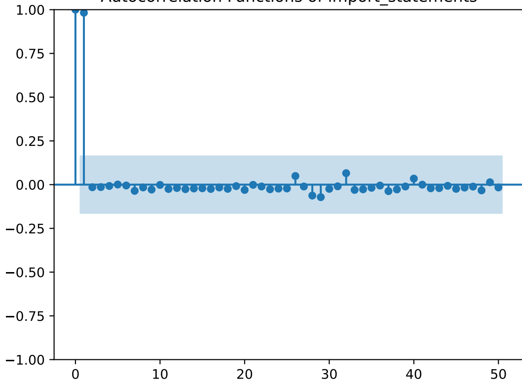
Autocorrelation Functions of import_statements
