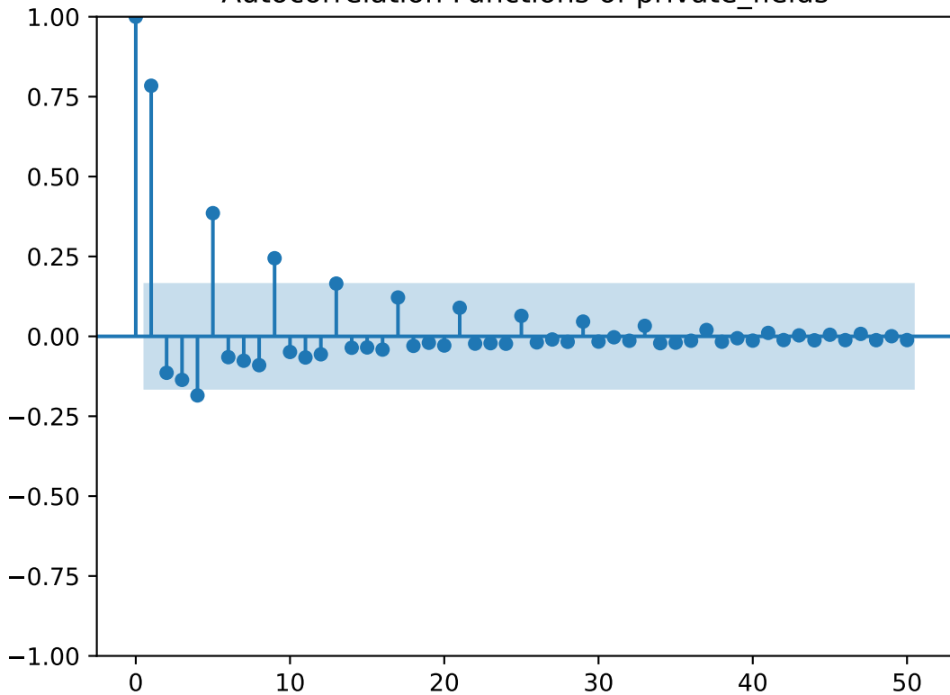
Autocorrelation Functions of private_fields
