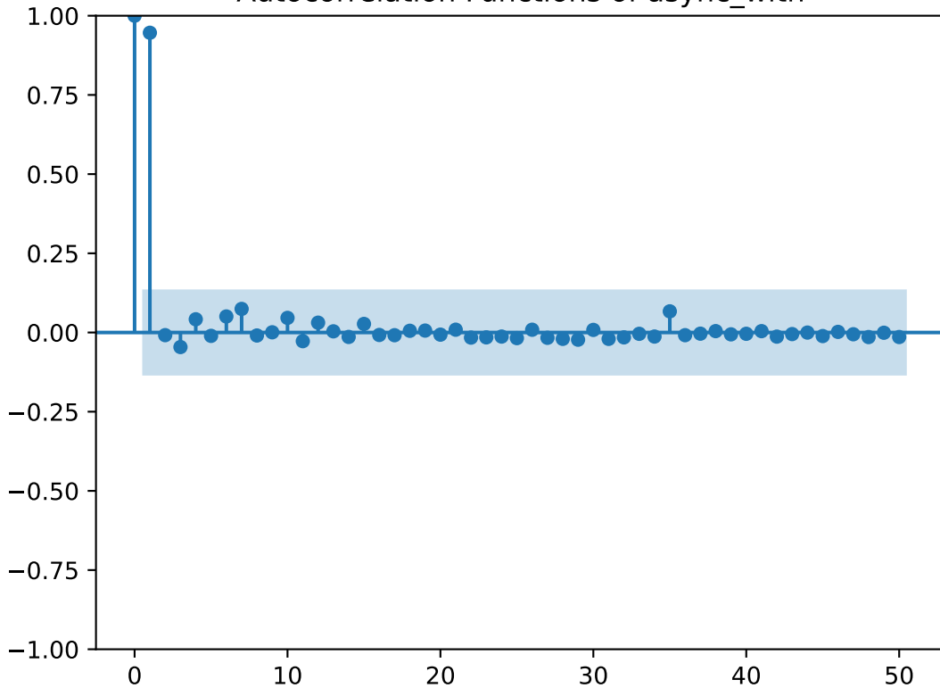
Autocorrelation Functions of async_with
