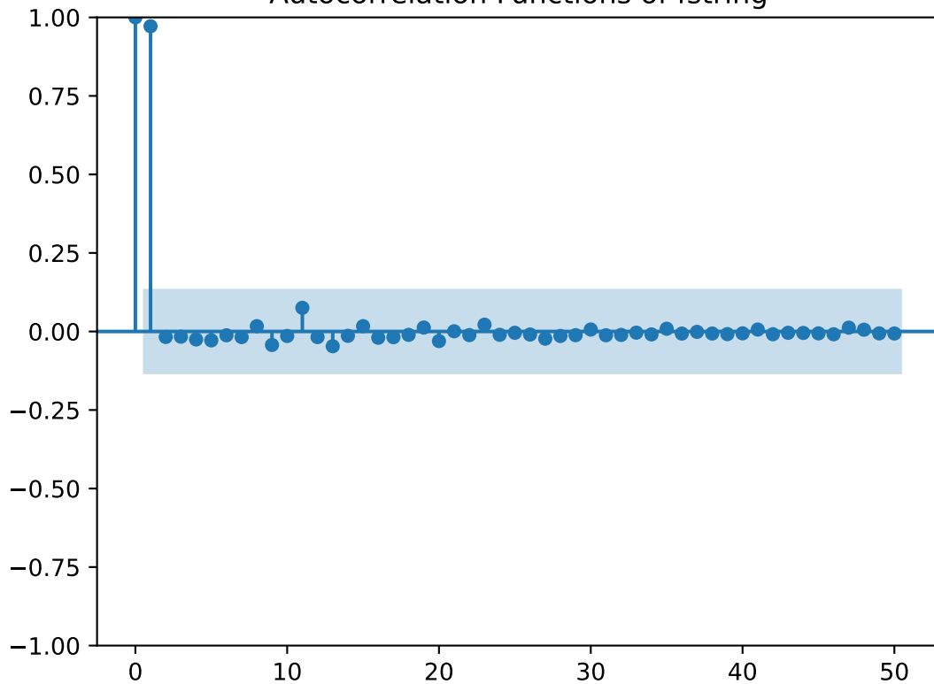
Autocorrelation Functions of fstring
