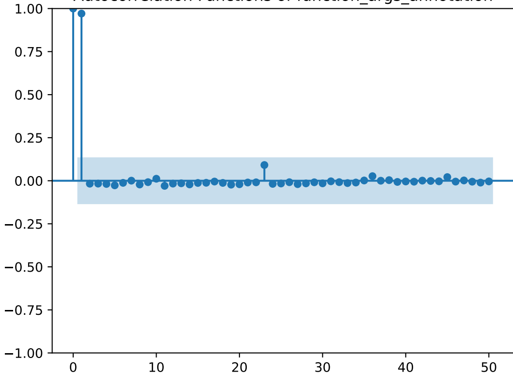
Autocorrelation Functions of function_args_annotation
