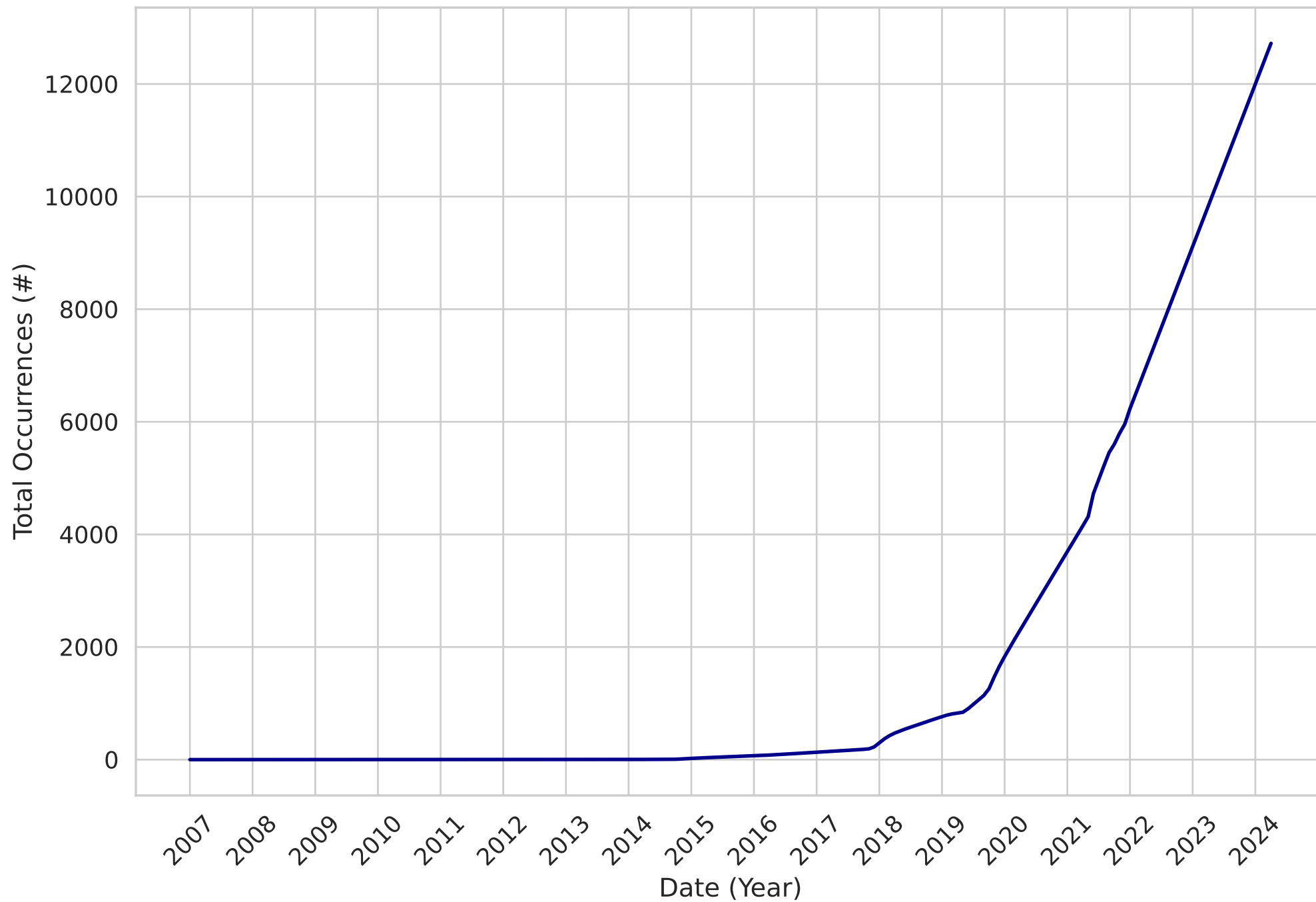
Function Return Annotation Files Trend
