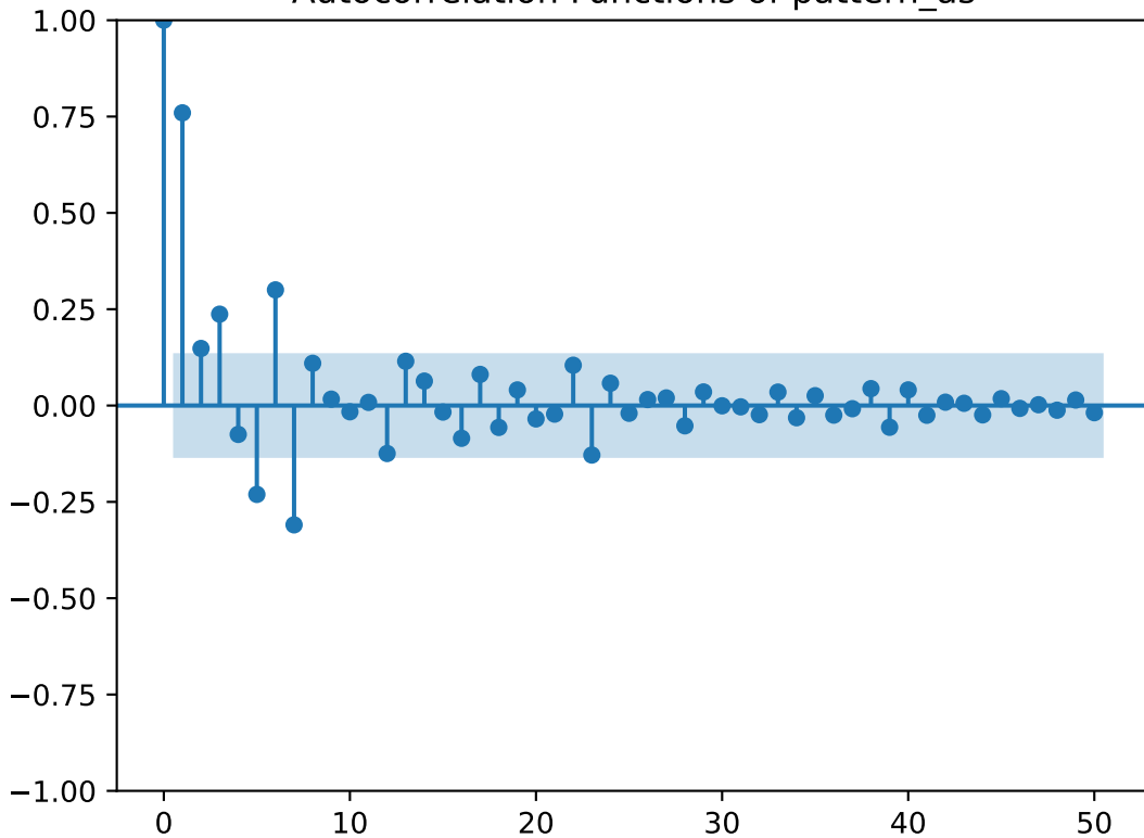
Autocorrelation Functions of pattern_as
