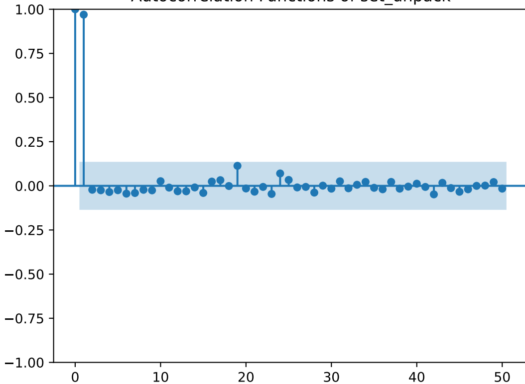
Autocorrelation Functions of set_unpack
