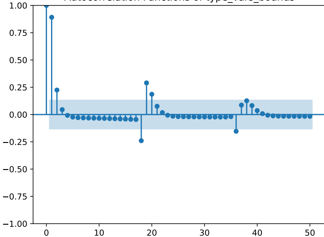
Autocorrelation Functions of type_vars_bounds
