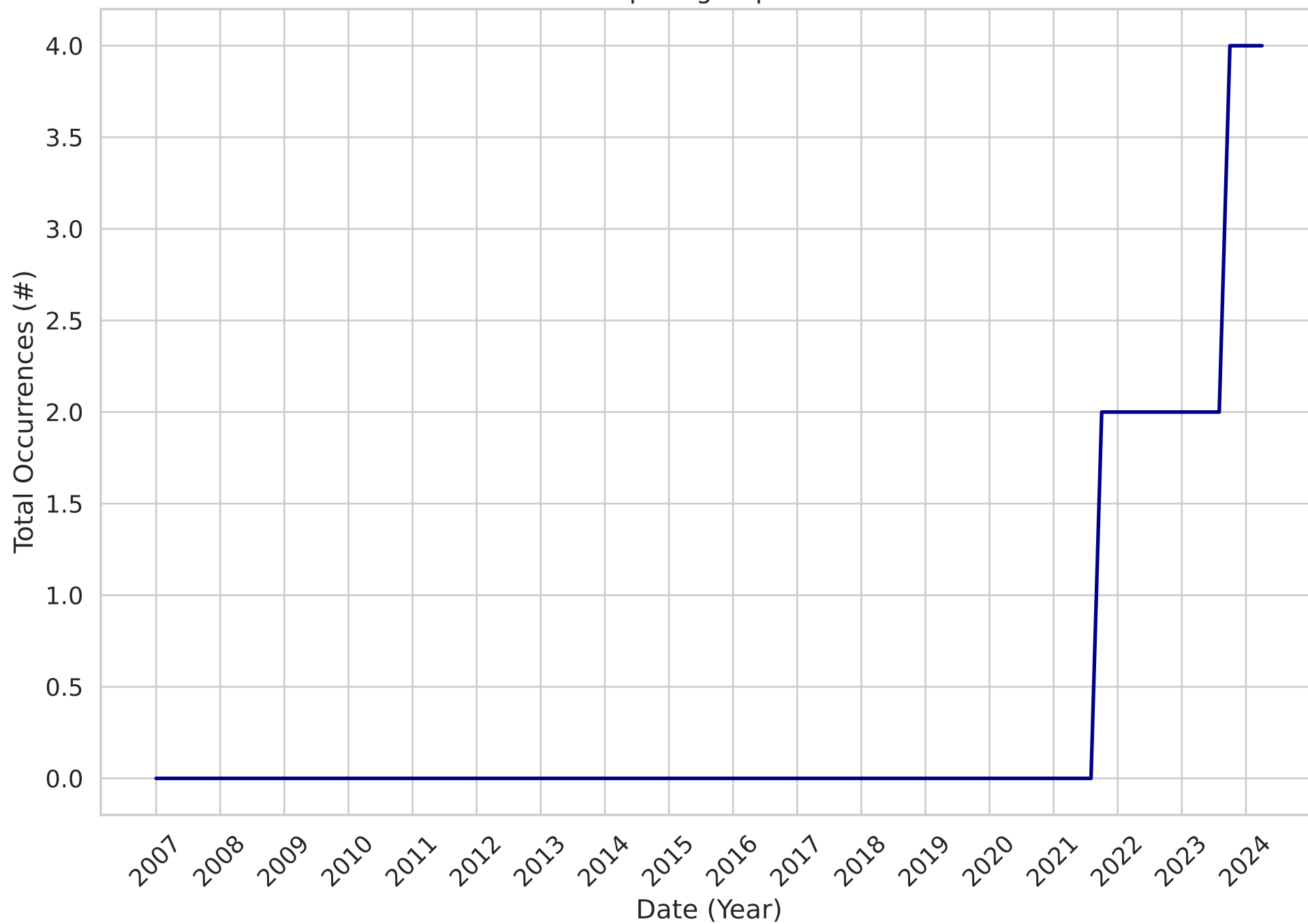
Exceptiongroup Trend
