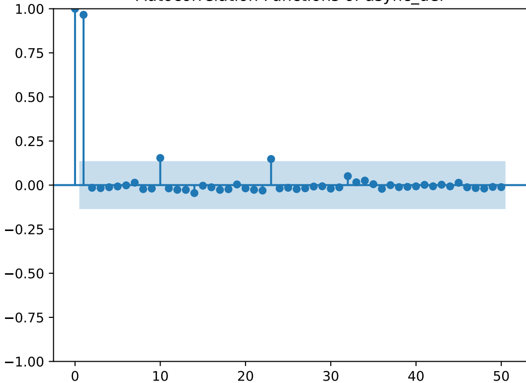
Autocorrelation Functions of async_def
