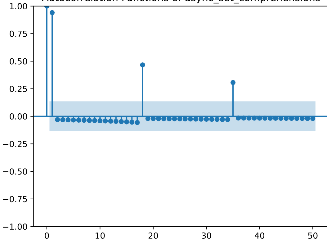
Autocorrelation Functions of async_set_comprehensions
