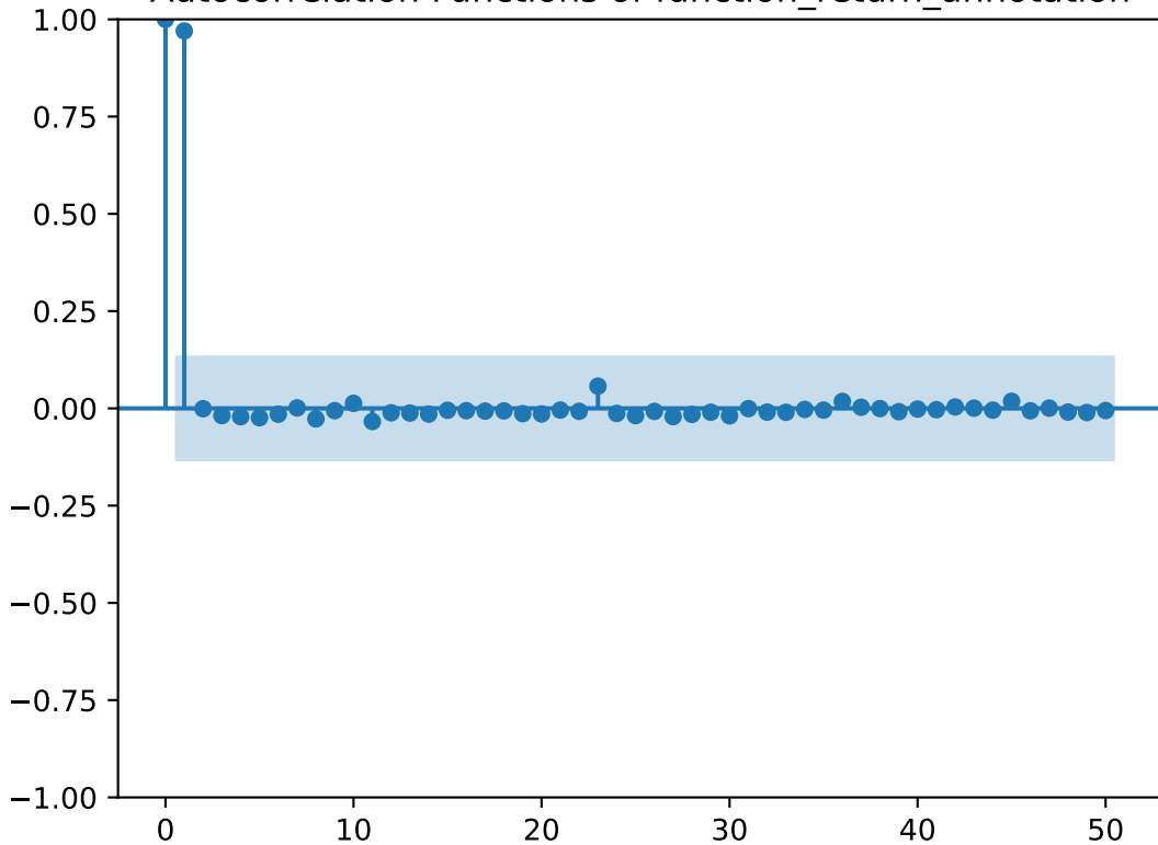
Autocorrelation Functions of function_return_annotation
