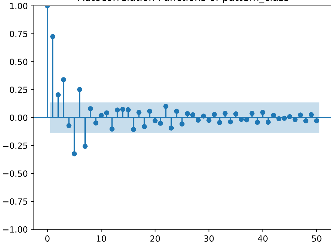
Autocorrelation Functions of pattern_class
