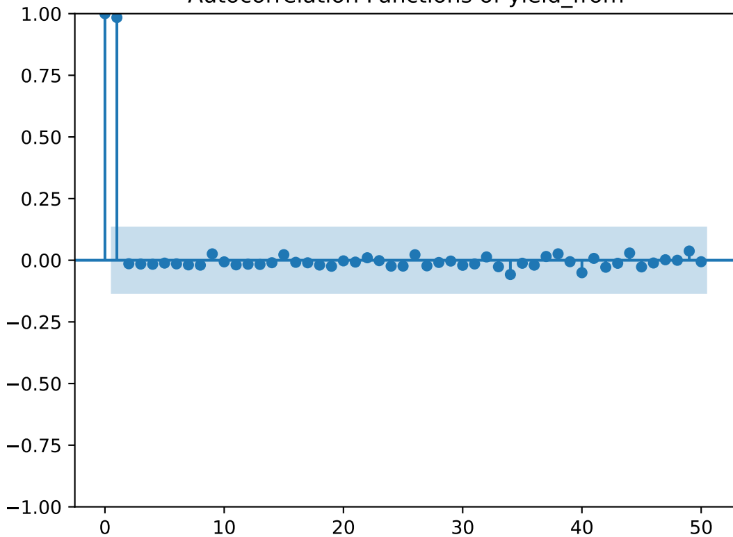
Autocorrelation Functions of yield_from
