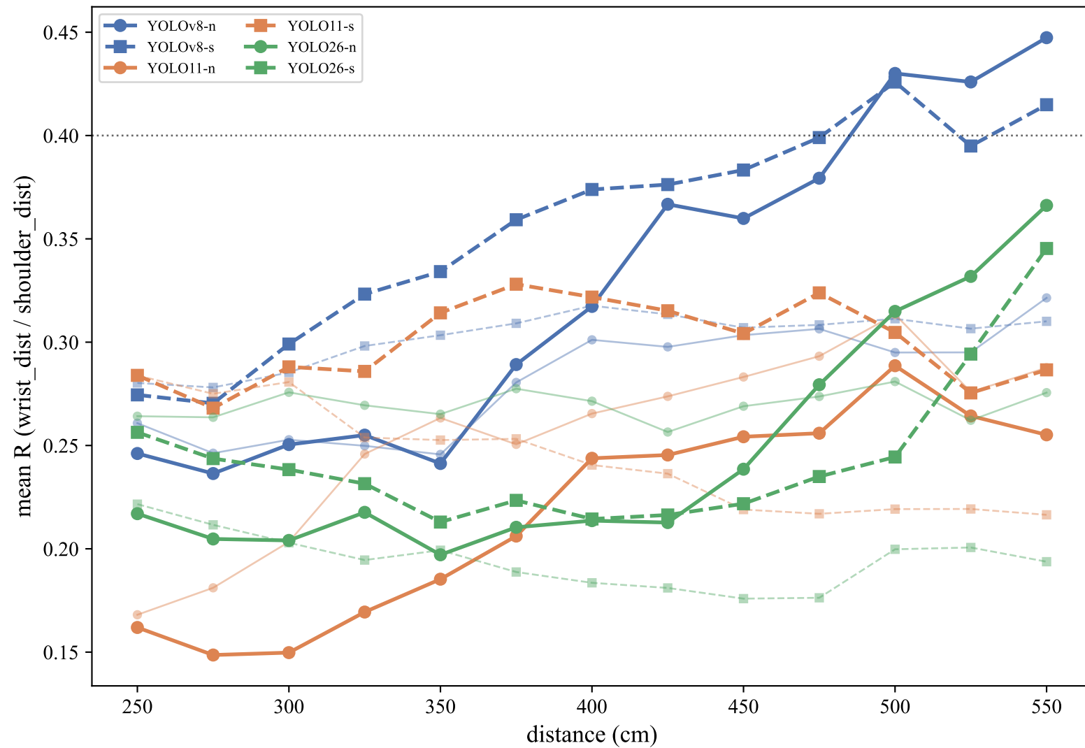
INT8(ModelOpt full)
