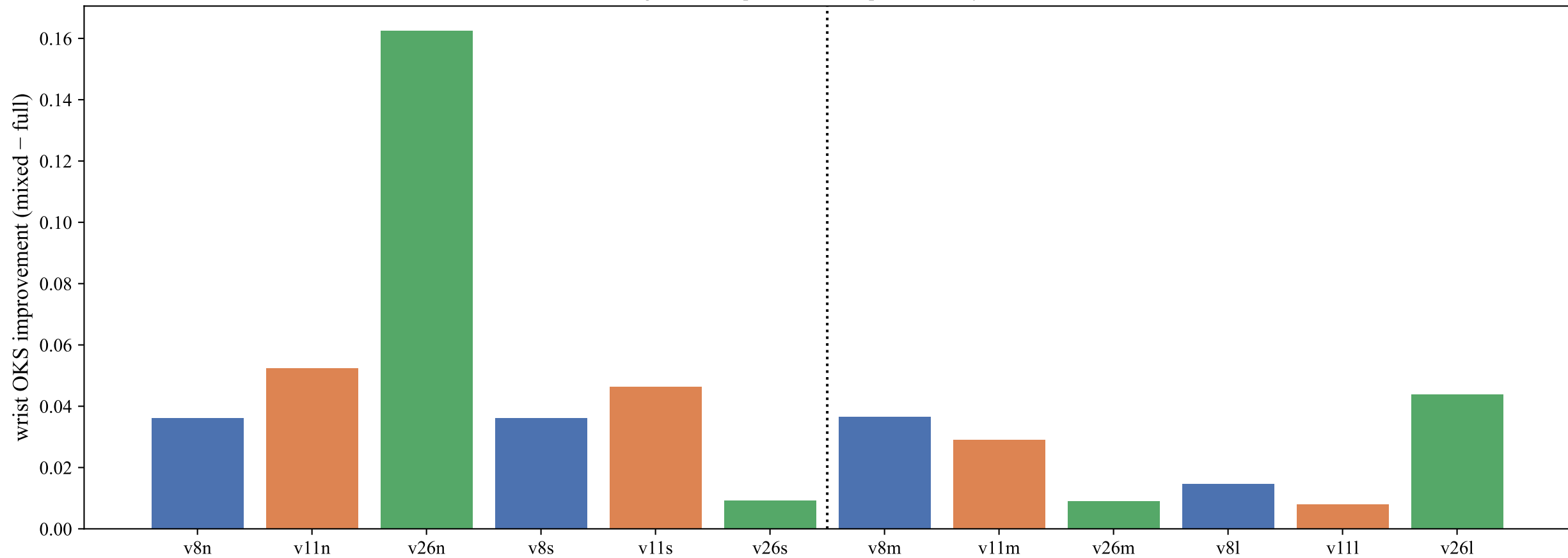
1-4: does excluding cv4 from quantization help consistently across all 12 models?
