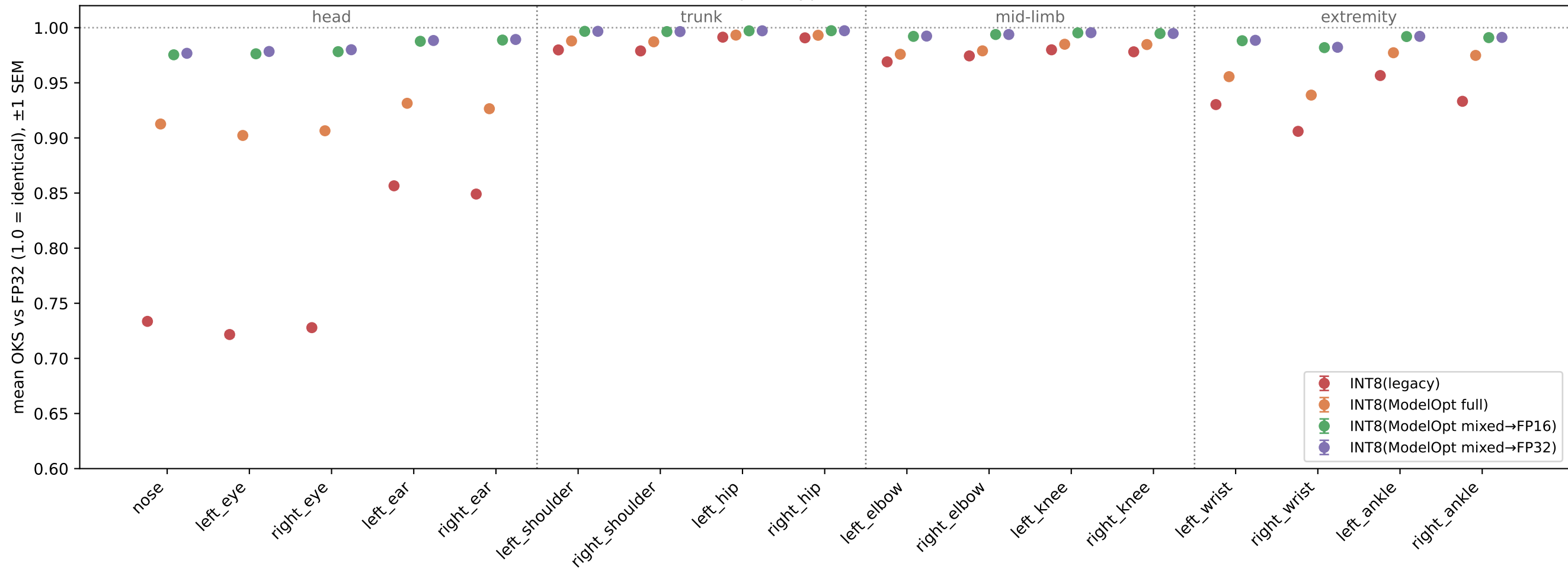
1-2 (hands-down): per-keypoint OKS vs FP32, 4 variants
