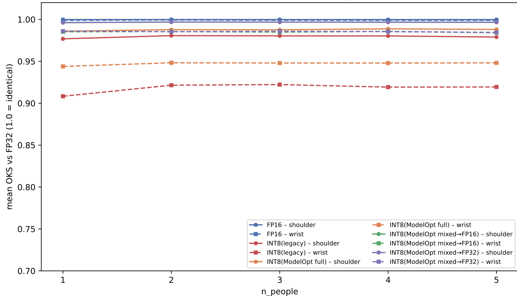
1-2 (hands-down): shoulder & wrist OKS vs n_people, 5 variants
