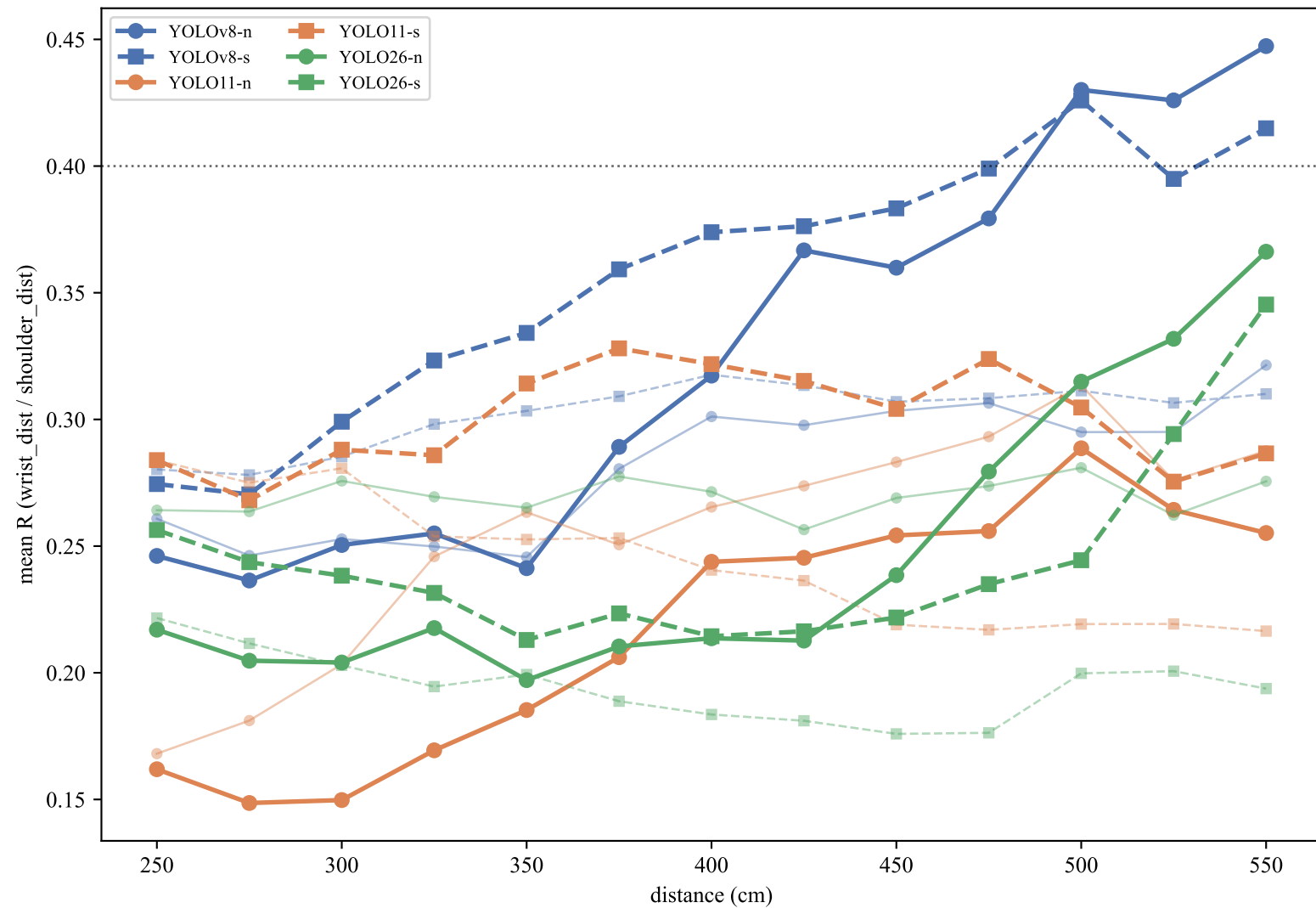
INT8(ModelOpt full)
