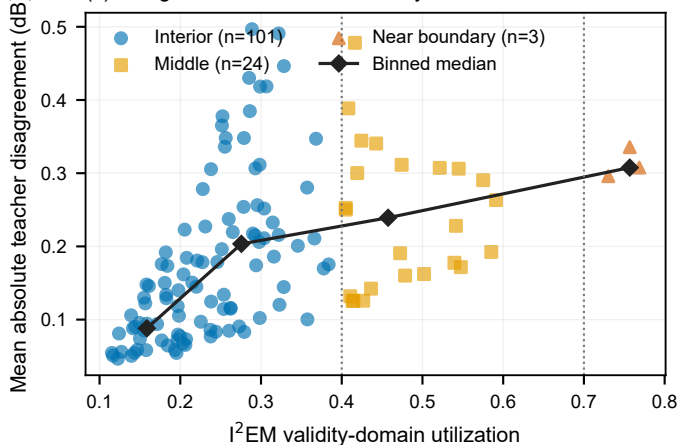
(c) Disagreement across the validity domain
