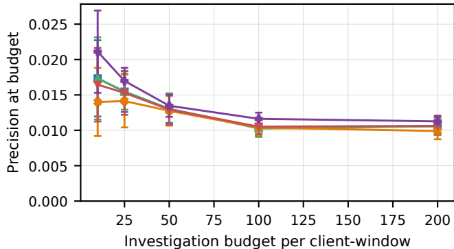
IBM AMLworld
