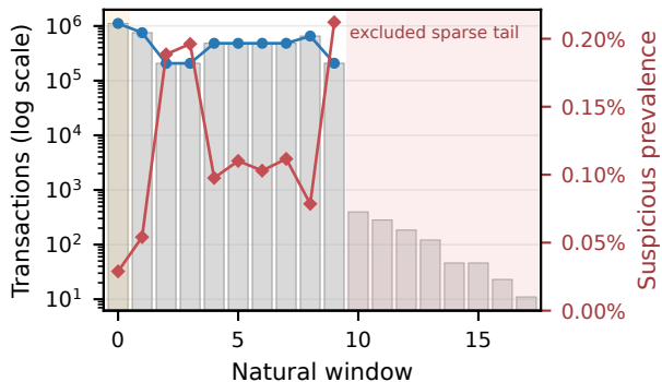
IBM AMLworld
