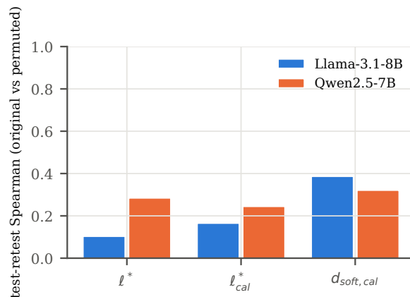
Figure 3: Reliability of the depth metrics on questions correct in both halves or orders. Source: CPU pilot (2,000 sampled questions, original and one permuted option order); to be replaced by the full run.
