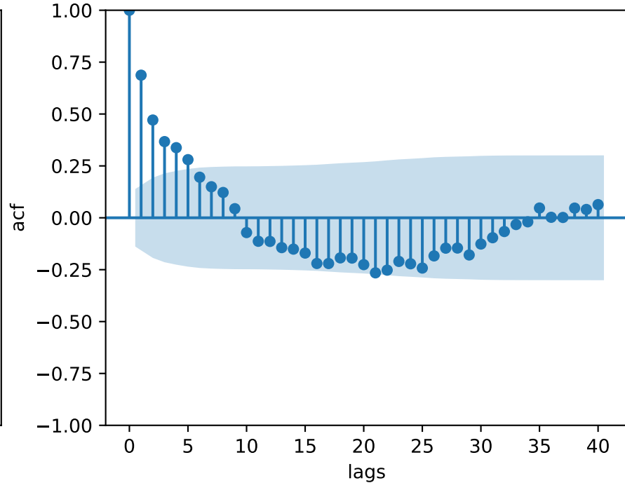
Autocorrelation
