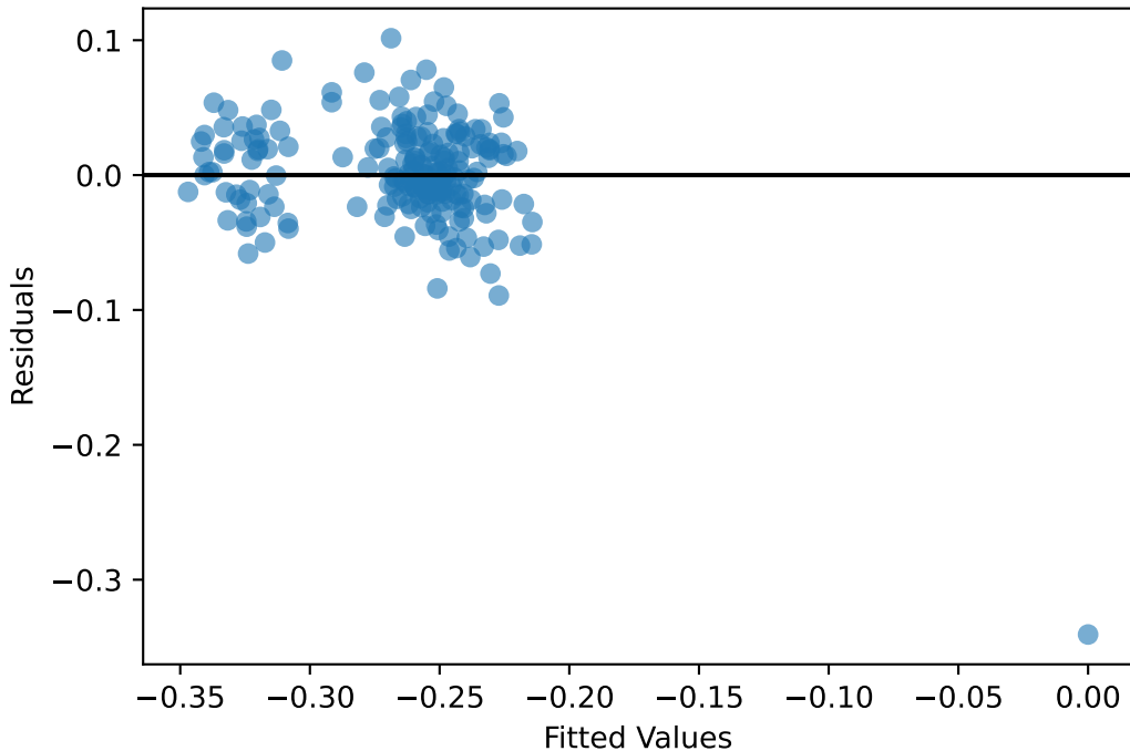
Base Variance of Residuals
