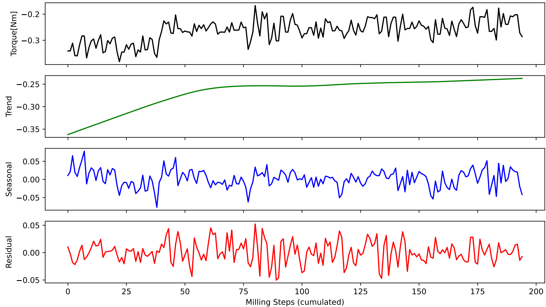
STL of Transformed Base Training Set
