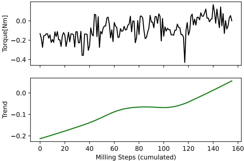
STL of Transformed Anomaly Training Set
