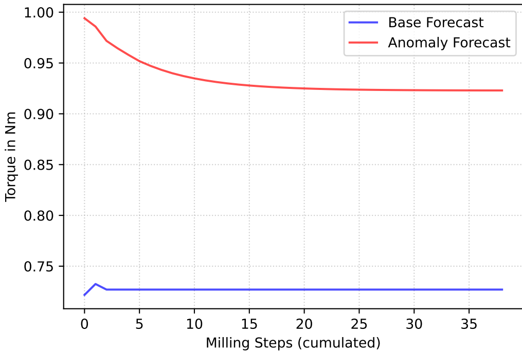
Base and Anomaly One Season ahead Forecast
