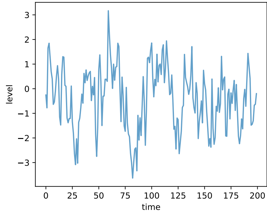
Time Series
