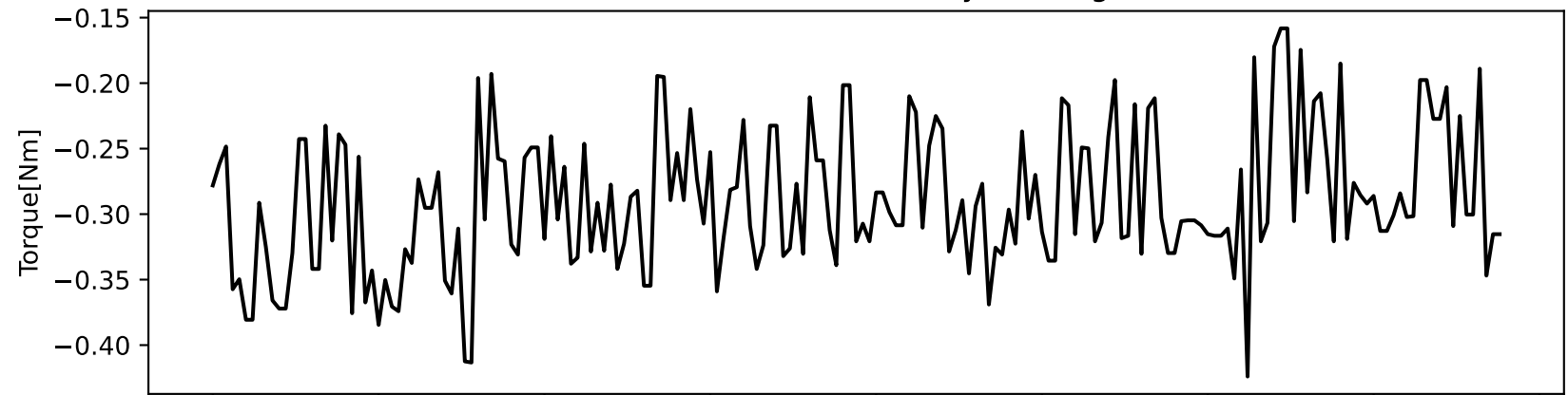
STL of Transformed Anomaly Training Set
