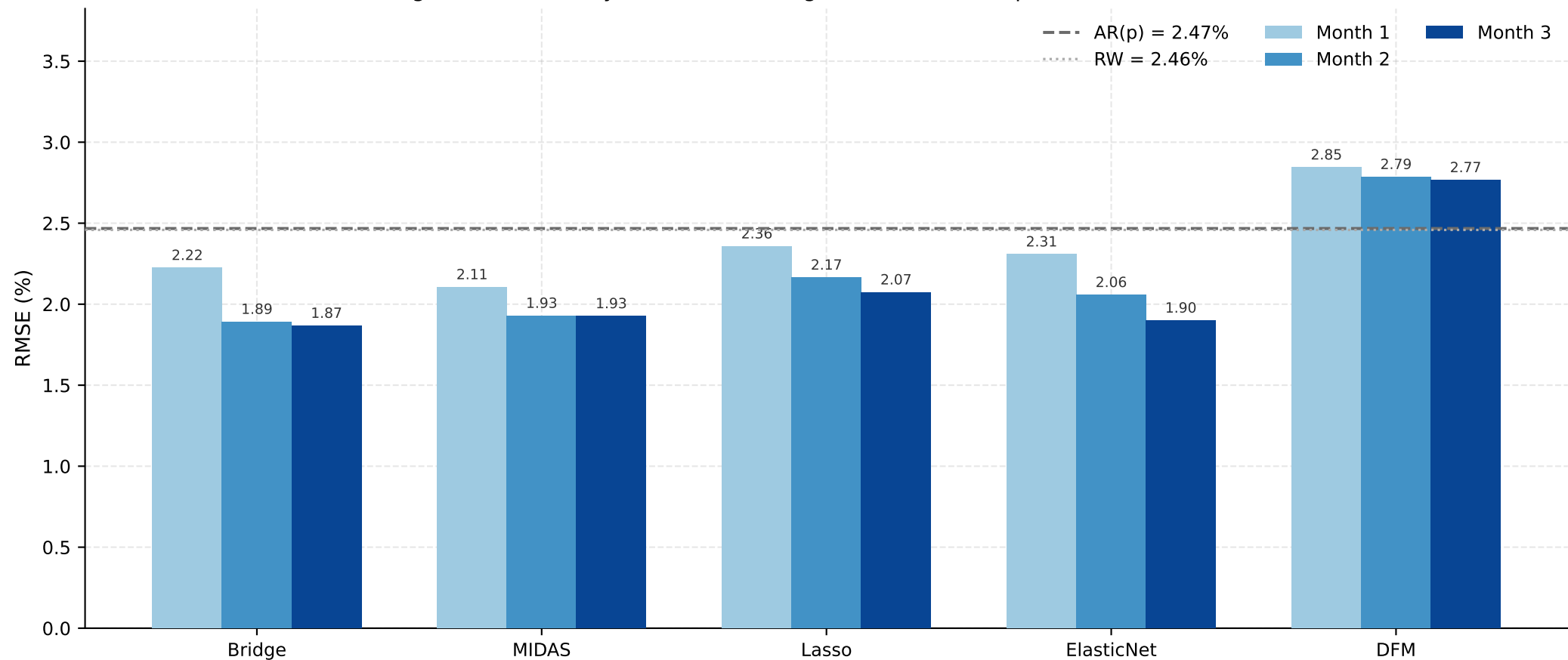
Figure 1 — RMSE by Model and Vintage (Pre-COVID sample, 2005Q1-2019Q4)
