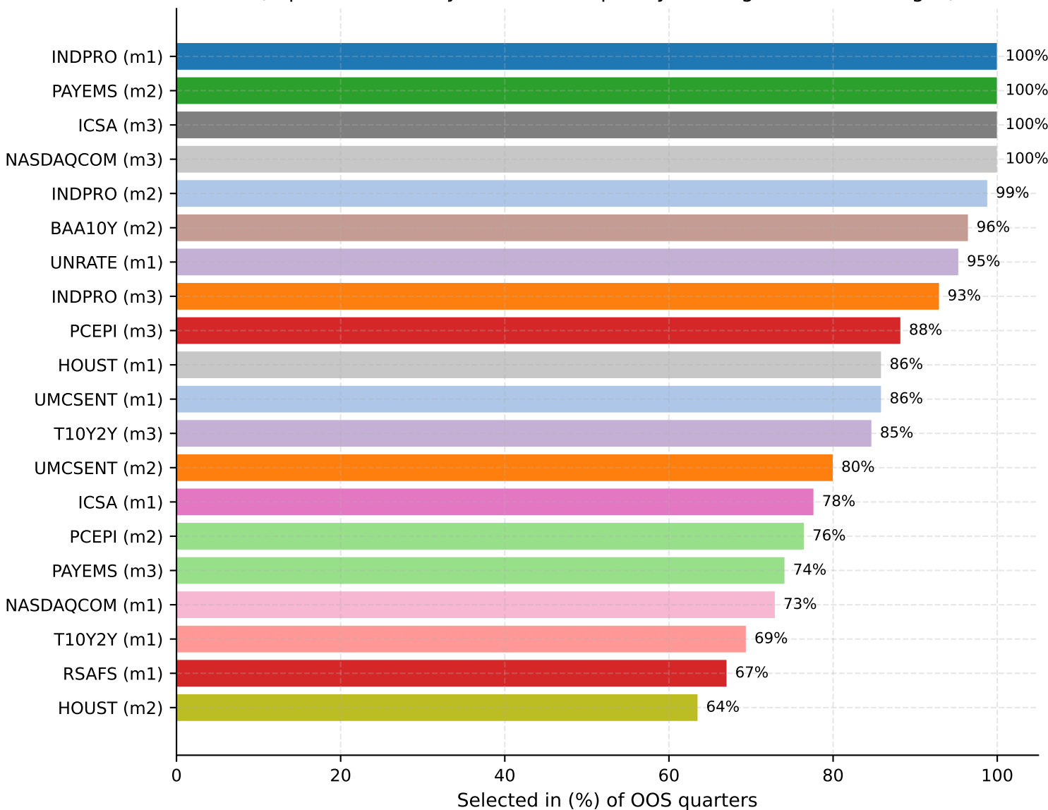
Figure 4 — Lasso Variable Selection Stability (Top 20 features by selection frequency, averaged across vintages)
