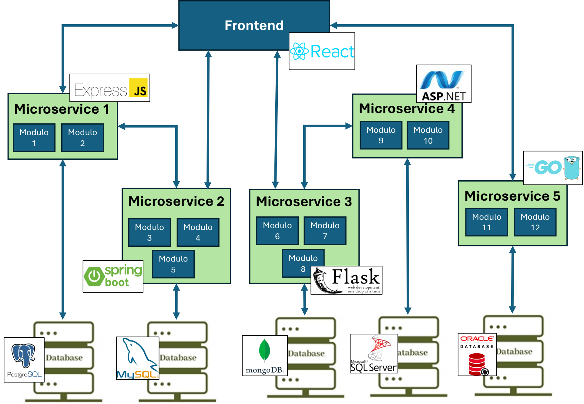
Microservices Architecture
