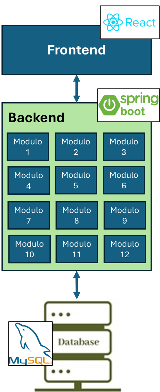
Monolithic Architecture
