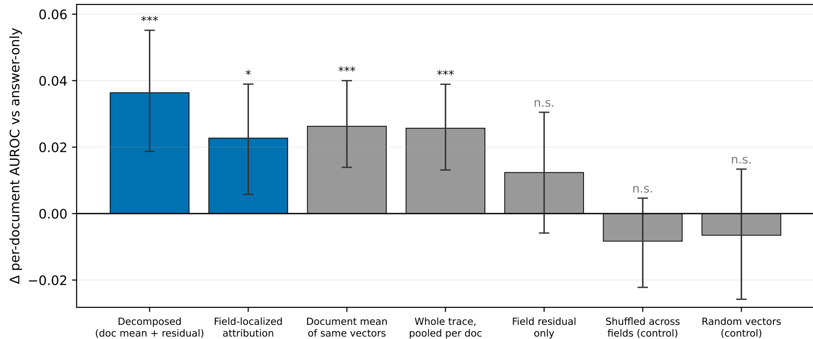
Reasoning variants vs the answer-only probe (layer 19) coloured = proposed, grey = control; 95% bootstrap CI over documents, Holm-corrected
