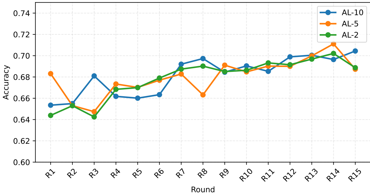
Accuracy Across AL Rounds ( \alpha = 0.01 )
