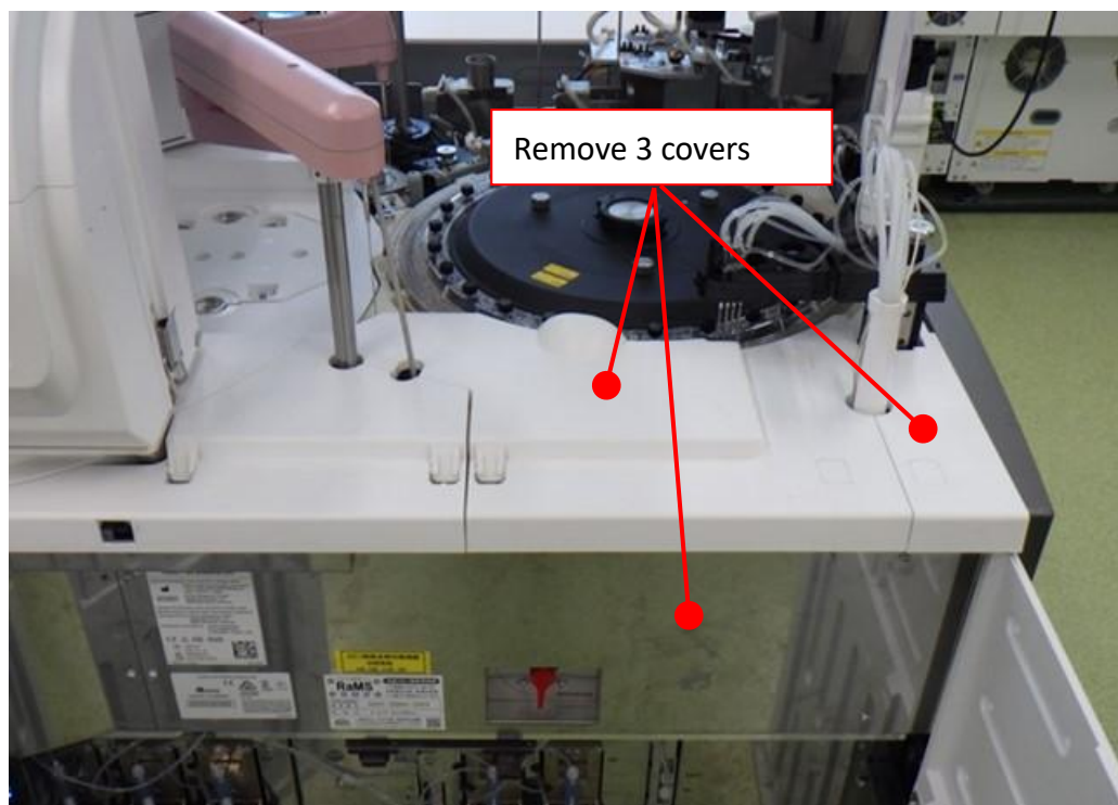
Fig. 24 Covers
