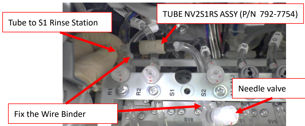
Fig. 28 Connect TUBE NV2S1RS ASSY
