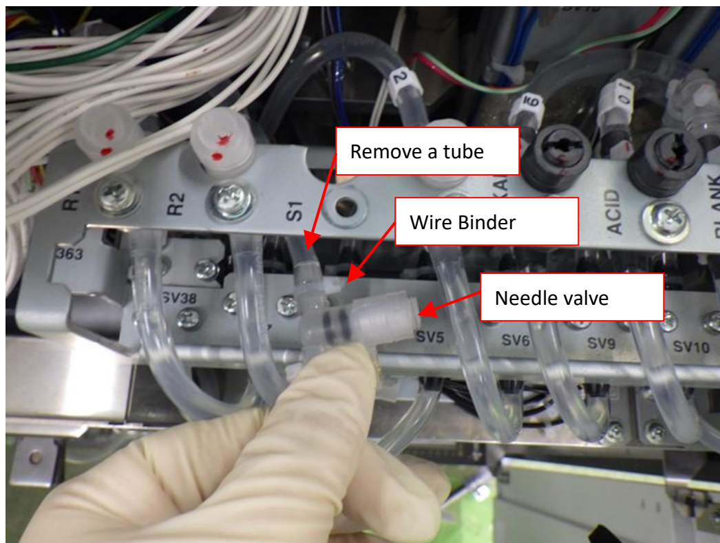
Fig. 26 Remove S1 needle valve
