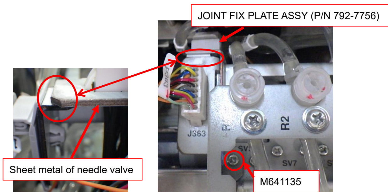
Fig. 30 JOINT FIX PLATE ASSY
