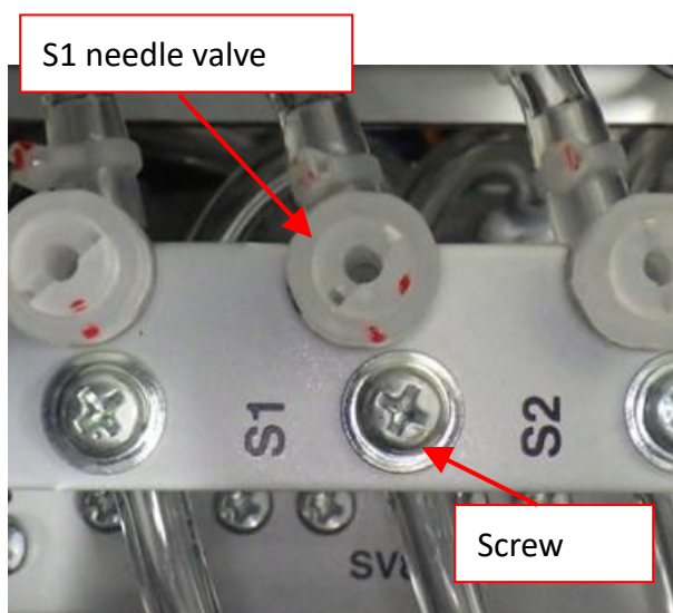
Fig.25 S1 needle valve
