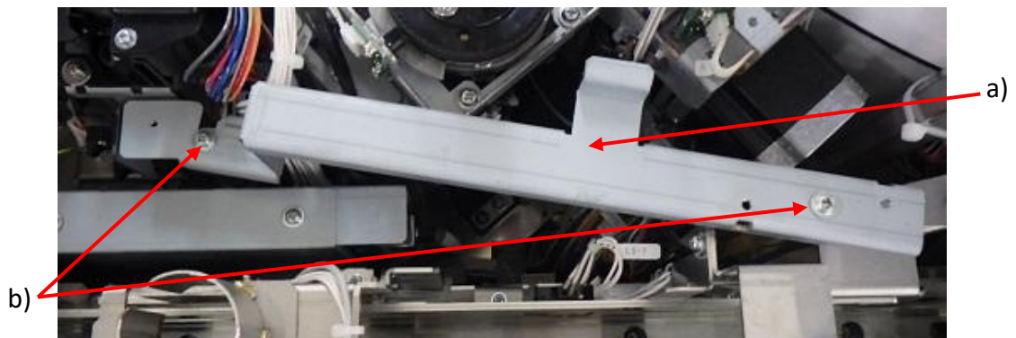
Fig.9 TB COVER FIXING PLATE 8
