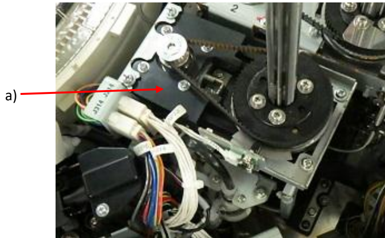
Fig.10 PIPETTER S1 ASSY
