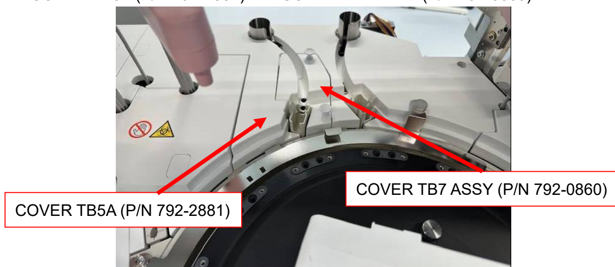
Fig. 34 Install COVER
