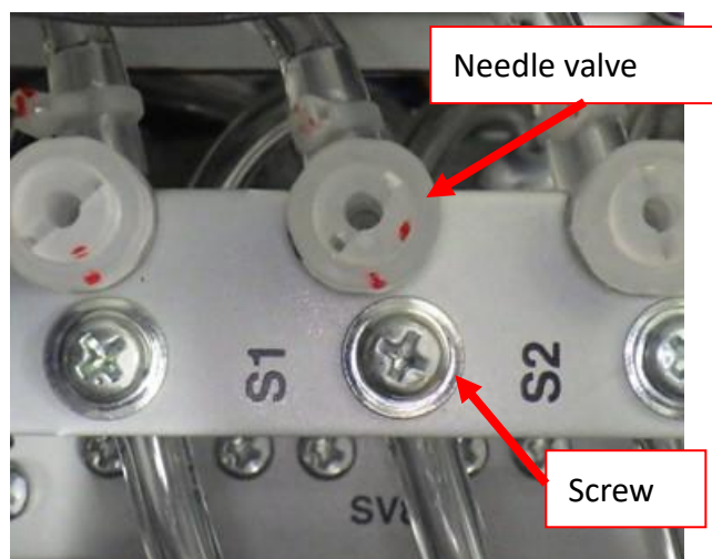
Fig. 31 Return the needle valve
