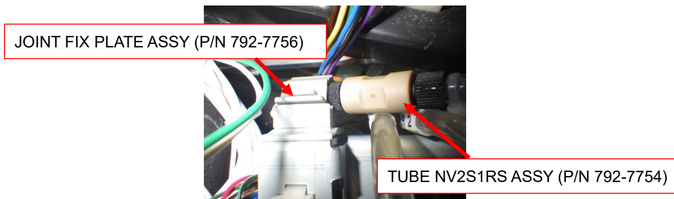
Fig.32 Clamping
