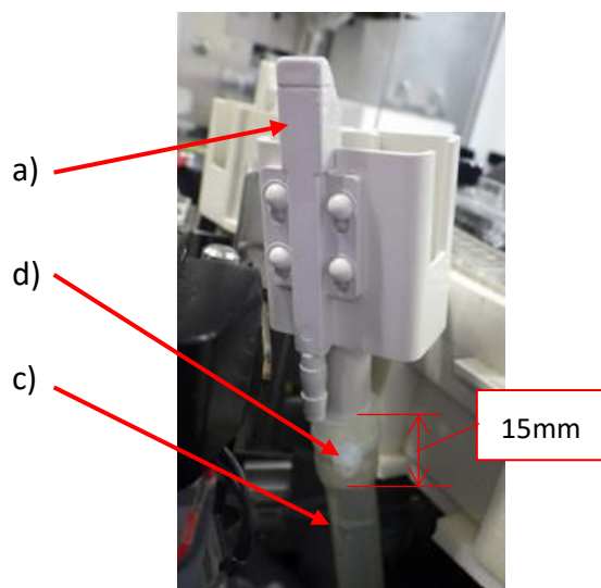
Fig.19 Drain tube
