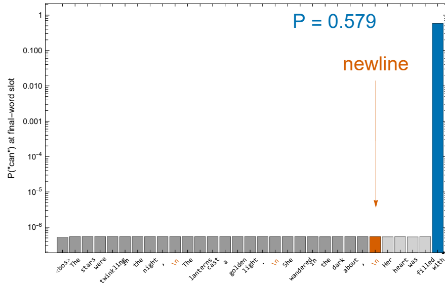
Gemma 2 2B × mntss 2.5M (word-level, s=10)
