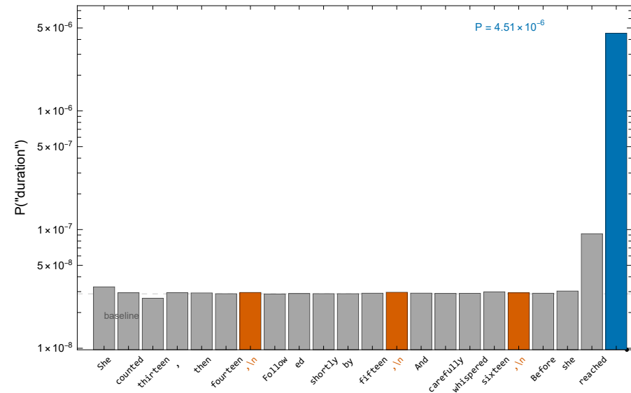
Qwen3-0.6B × BlueLightAI 20K (–teen → “duration”, s=1)
