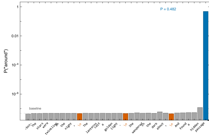
Gemma 2 2B × mntss 426K (–out → “around”, s=25)
