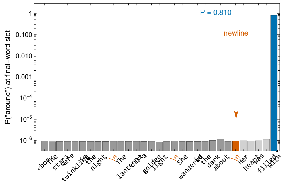
Gemma 2 2B × mntss 426K (group-level, s = 25)
