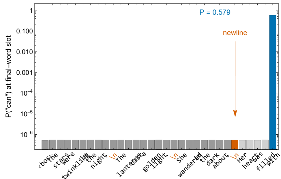
Gemma 2 2B × mntss 2.5M (word-level, s = 10)
