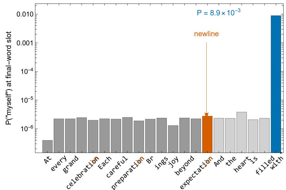
Qwen3-0.6B × BlueLightAI 16K (-ation, s = 25)
