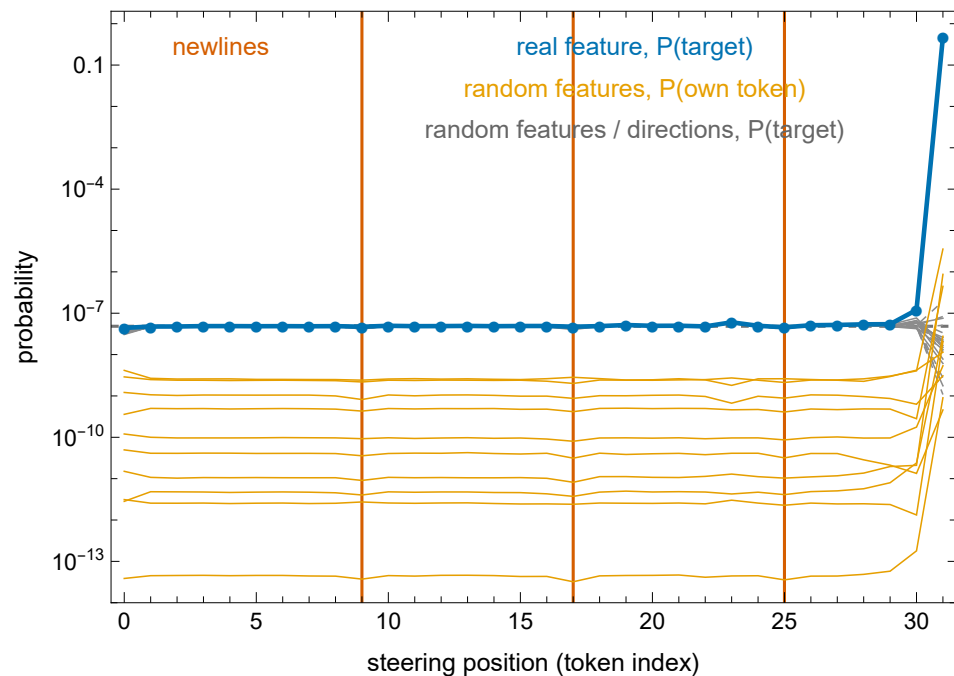
Qwen3-0.6B × BlueLightAI 16K (target “myself”, s = 25)
