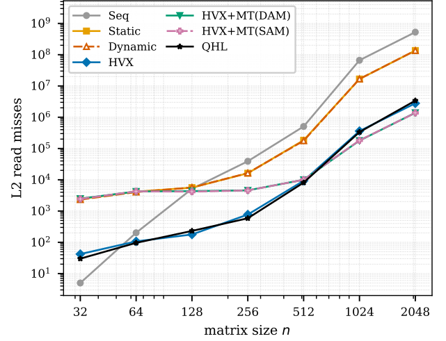
Fig. 8. L2 read misses vs. n (log-log), all seven variants. The scalar band (SEQ, STATIC, DYNAMIC) overflows L2 (SEQ reaches 5.3 \times 10^8 misses at n=2048 ); the vector variants (HVX, HVX+MT(DAM), HVX+MT(SAM)) and QHL stay two to three orders of magnitude lower, which is the source of the band split in Fig. 4.
