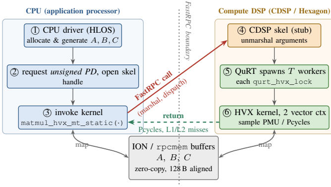
Fig. 2. One FastRPC offload from the CPU to the Hexagon compute DSP (CDSP). The host allocates shared rpcm /ION buffers, opens the DSP skel, and invokes the kernel through FastRPC. On the DSP, the skel unmarshals the arguments, QuRT launches worker threads, and each worker acquires an HVX context before executing the vector kernel. Since the input and output buffers are shared between the CPU and DSP, data is transferred without copying, and only the performance counters are returned to the host.
