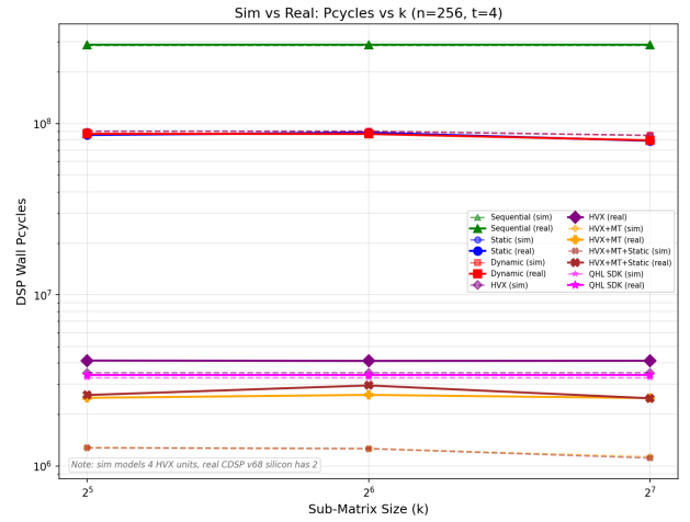
Fig. 11. Pcycles vs tile size for both simulator and real soc
