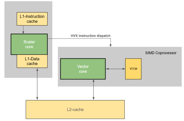
Fig. 1. Memory organisation of the Hexagon DSP. The scalar core owns private L1 instruction and data caches, while the HVX coprocessor reads and writes through its own path and a dedicated VTCM scratchpad; both sides meet at the shared L2 cache, which serves as the vector unit’s first-level memory.
