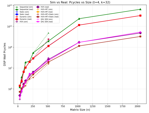
Fig. 10. Pcycles vs matrix size for both simulator and real soc
