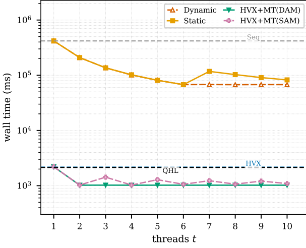
Fig. 6. Thread scaling, wall-clock time ( n=1024 , k=32 , log y ). Scalar STATIC and DYNAMIC scale to t \approx 6 (six hardware threads); HVX+MT(DAM) and HVX+MT(SAM) saturate at t=2 (two HVX contexts). STATIC and HVX+MT(SAM) show the SAM load-imbalance cliff when t does not divide the 1024-block grid; DYNAMIC and HVX+MT(DAM) stay flat. SEQ, HVX, and QHL are thread-independent and shown as horizontal reference lines at their single measured value ( t=4 ).
