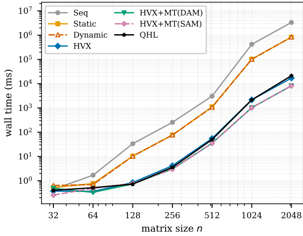
Fig. 4. Wall-clock time vs. matrix size (log-log). The scalar variants form a slow band; the vector variants and QHL cluster in a fast band. HVX+MT(DAM) leads the fast band for n \geq 128 . Ranking below n=128 is noisy; see Section IV-G.
