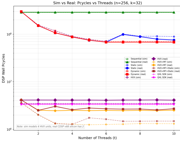
Fig. 12. Cycles vs threads for both simulator and real soc
