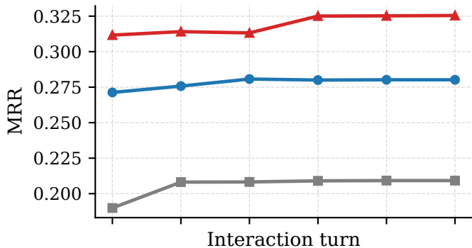
MRR
